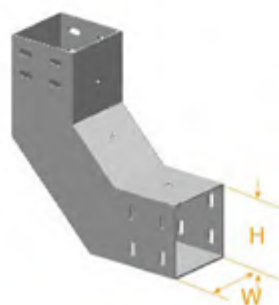
BT1/2/3/4/5/6 -IR Inside Riser
