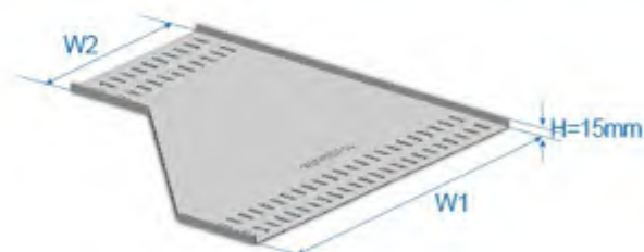
BC1-MR Middle Reducer
