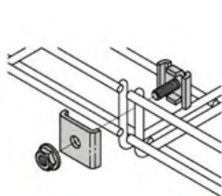
WB4CA Connector Assembly
