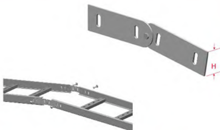
BL1/2/3-VAC N12B/16A/20B/20C-VAC Vertical Adjust Coupler
