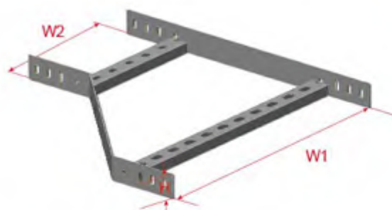
BL2-RR Right Hand Reducer
