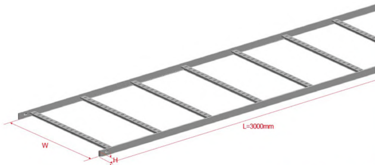
MCL Marine Cable Ladder
