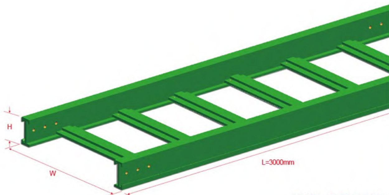
BL5/6 Cable Ladder
